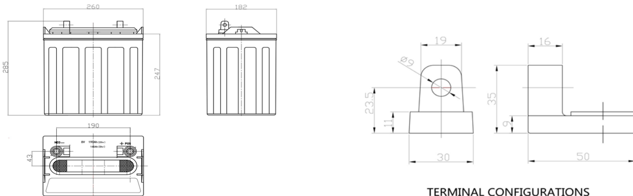
TERMINAL CONFIGURATIONS
